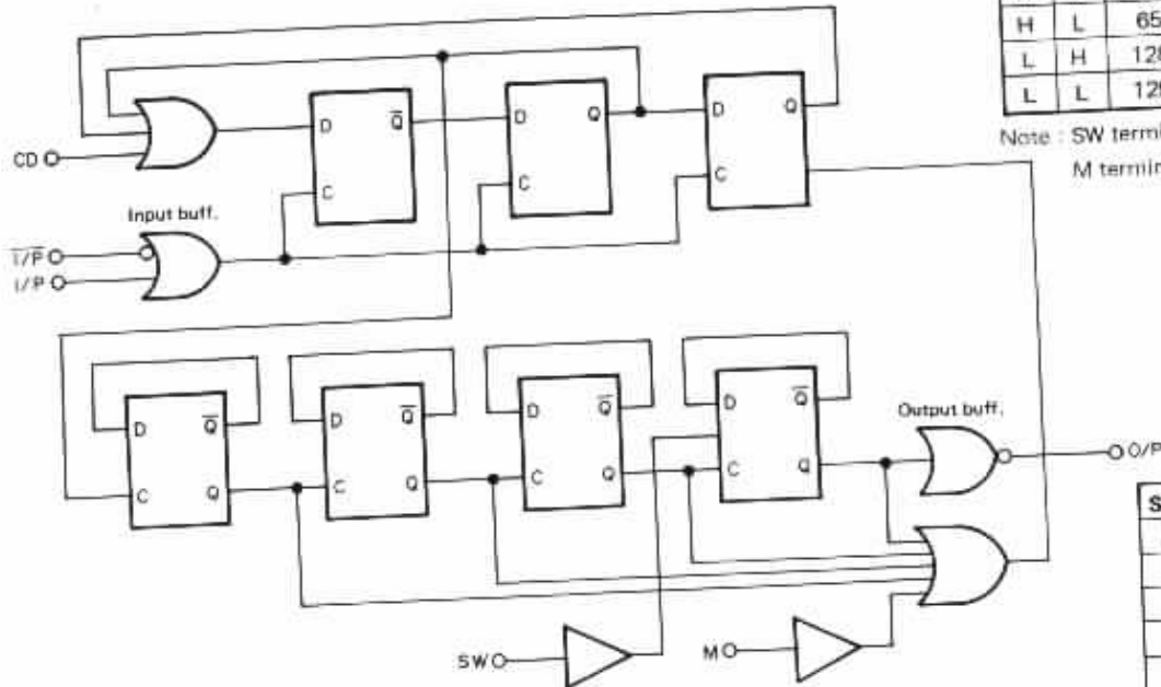
MB501P/MB504P (COMPOSITE UNIT (PLL-TX) Q19,25) • Block diagram
