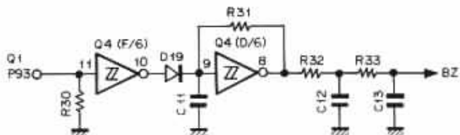
Fig. 9 Beep circuit
