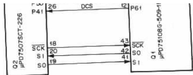
Fig. 7 Interfacing of microprocessors
