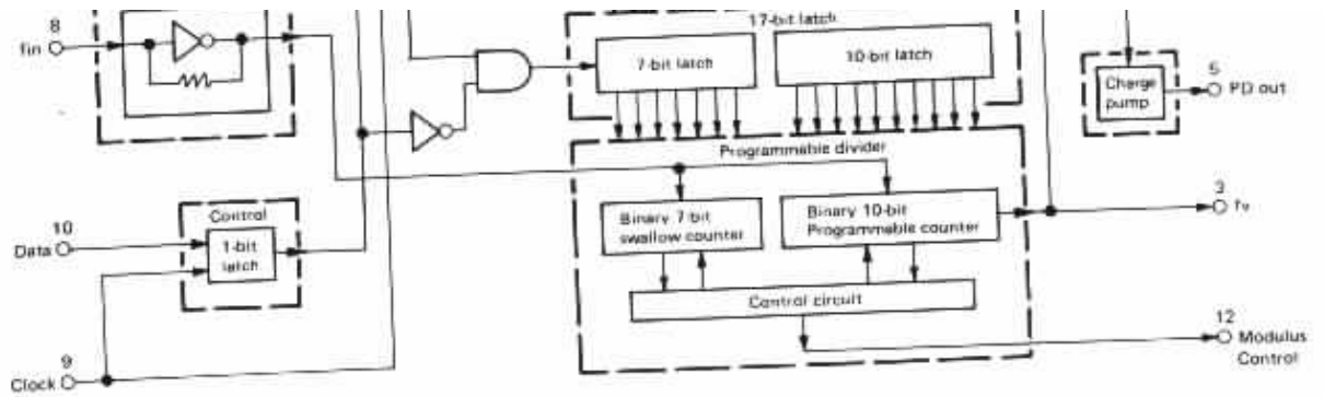
MB501P/MB504P (COMPOSITE UNIT (PLL-TX) Q19,25) • Block diagram
