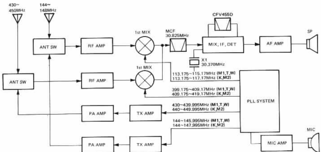
Fig. 1 Block diagram showing frequencies
